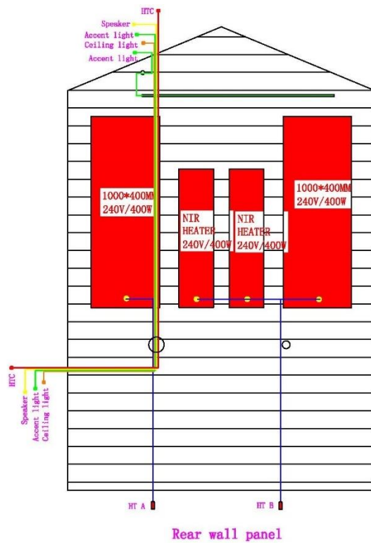
Rear wall panel
