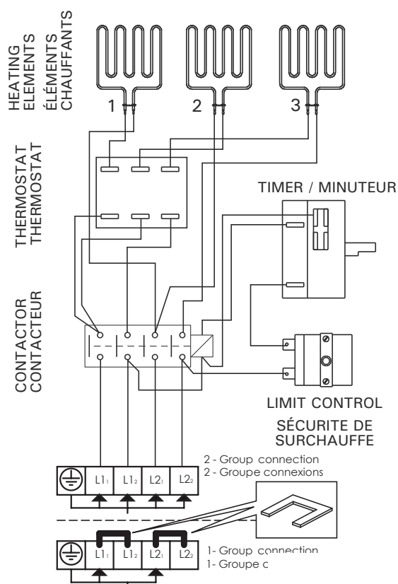
Figure 5. Electrical connections of the heater
