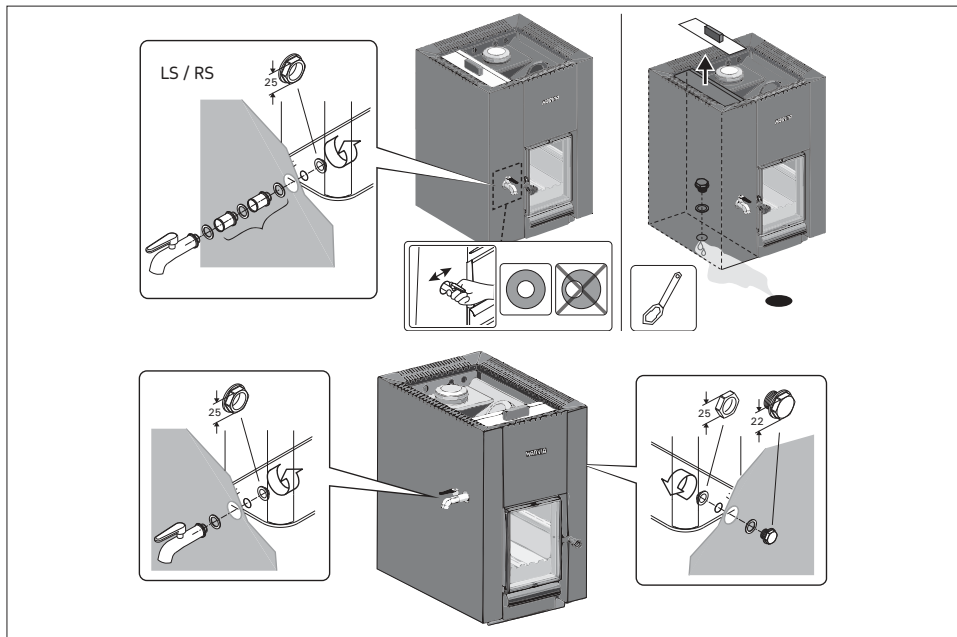
Figure 3. Mounting the water tap.
